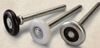
Black nylon, white nylon, 10 ball steel roller
